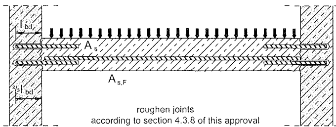
Figure 3: End anchorage of slabs or beams, designed as simply supported
