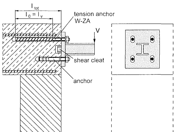
Figure 8: Overlap joint for the anchorage of a cantilevers
